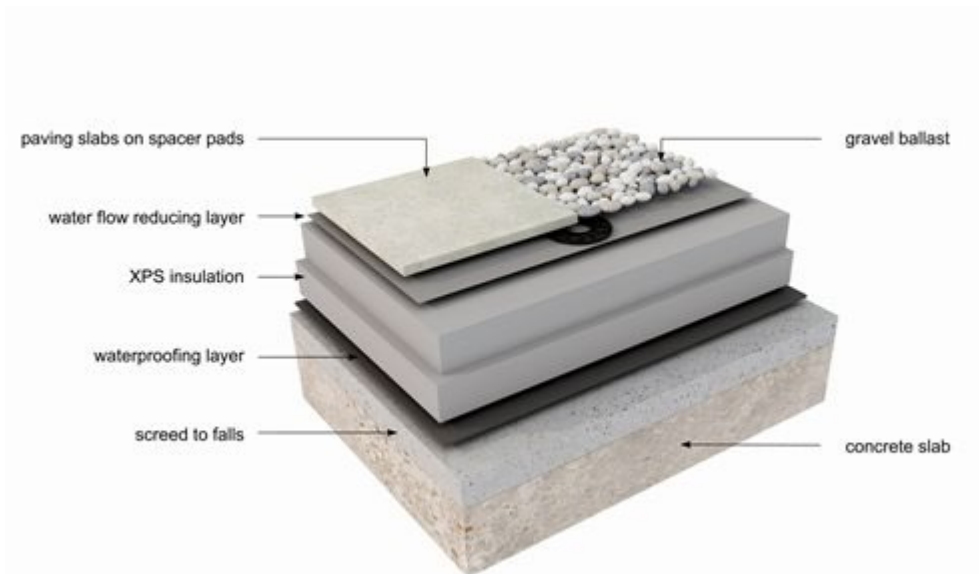
Figur 10: Flatt tak
